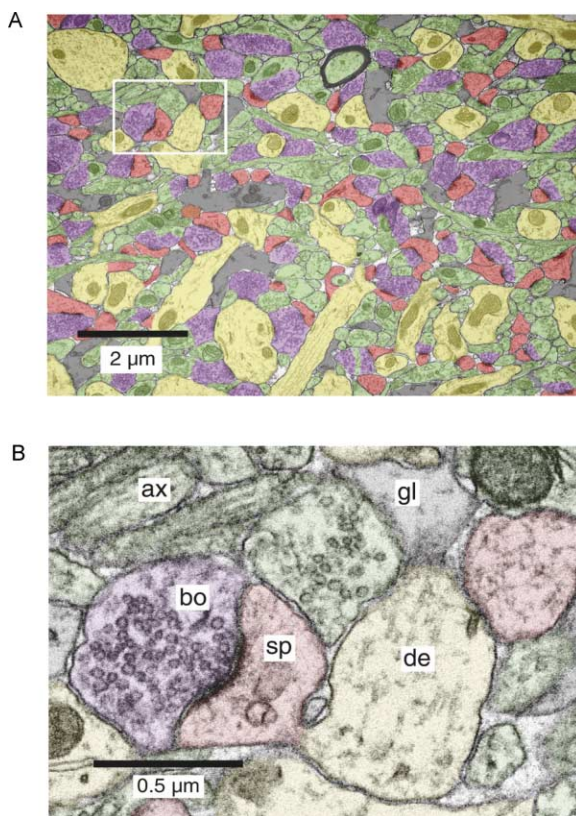
Figure 2. Electron Micrograph of Hippocampus (CA1) to Illustrate the Fraction of Different Components
