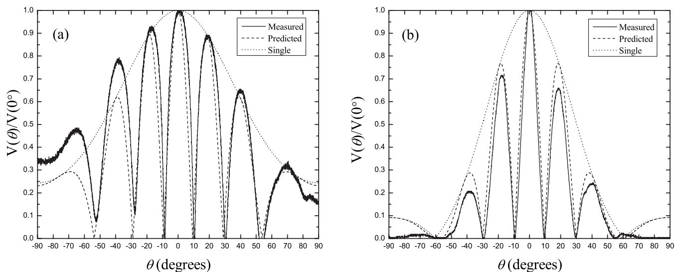
Fig. 5. The far-field beam pattern functions for (a) two 25 kHz transmitters ( d/\lambda = 3.1 \pm 0.1 ) and (b) two 40 kHz transmitters ( d/\lambda = 3.00 \pm 0.05 ). The validity of the product theorem is demonstrated by the single baffled circular piston source pattern, labeled "single," which bounds the two-source patterns.
