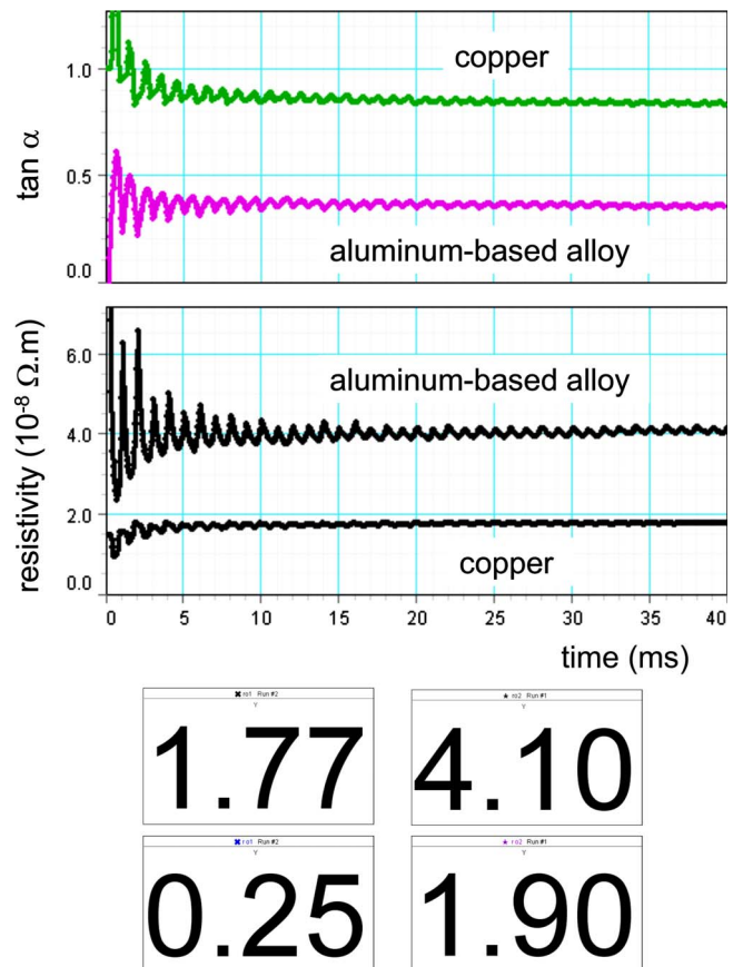
Fig. 3. The averaging process and digital displays of the resistivity of copper and an aluminum-based alloy at room and liquid nitrogen temperatures.
