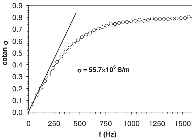
Fig. 4. Results of the measurements of the electrical conductivity in a lathed copper rod with a radius of 5.56 mm. The probe coil used was a monolayer coil of very thin copper wire carefully arranged on the surface of the rod. The straight line corresponds to the low-frequency approximation while the curve represents the numerical simulation at higher frequencies. The error bars are smaller than the size of the data points.
